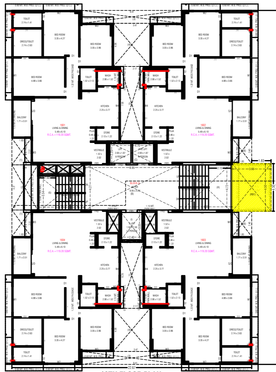
16TH.FLOOR PLAN
