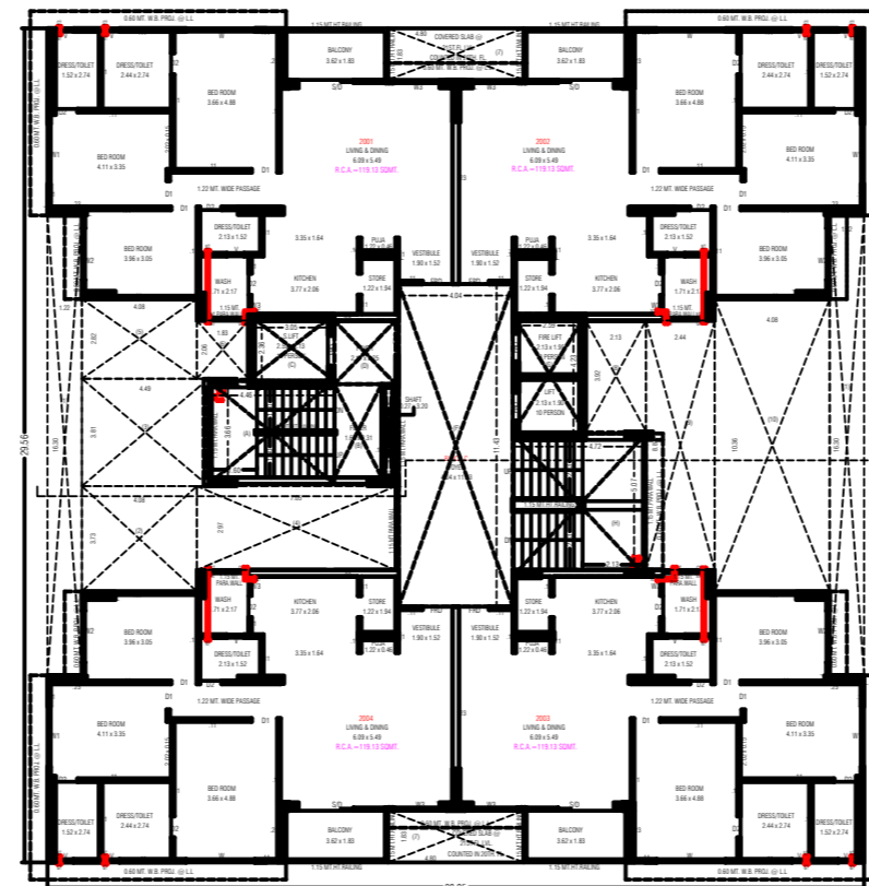
20TH FLOOR PLAN
