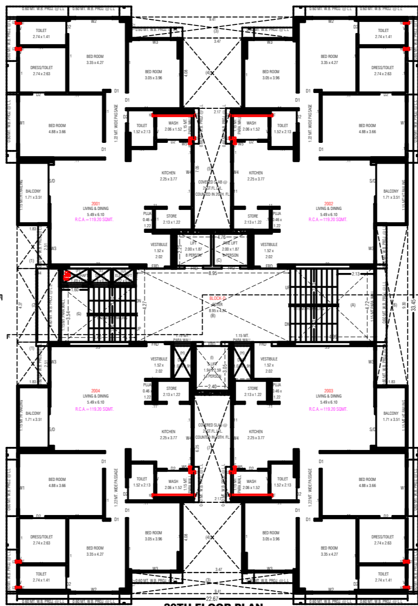
20TH.FLOOR PLAN
