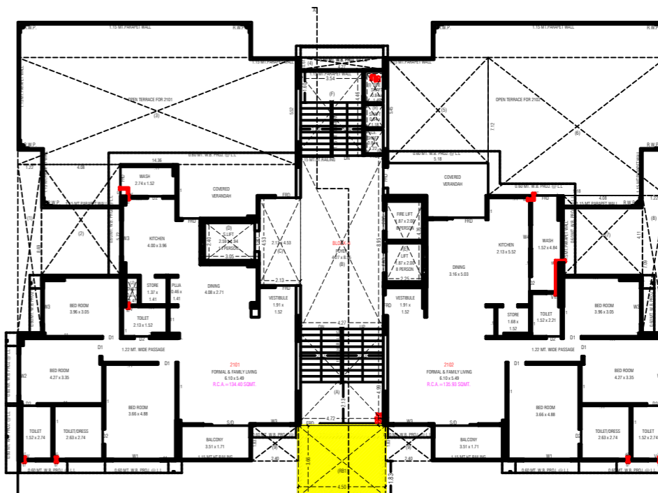
21ST.FLOOR PLAN
